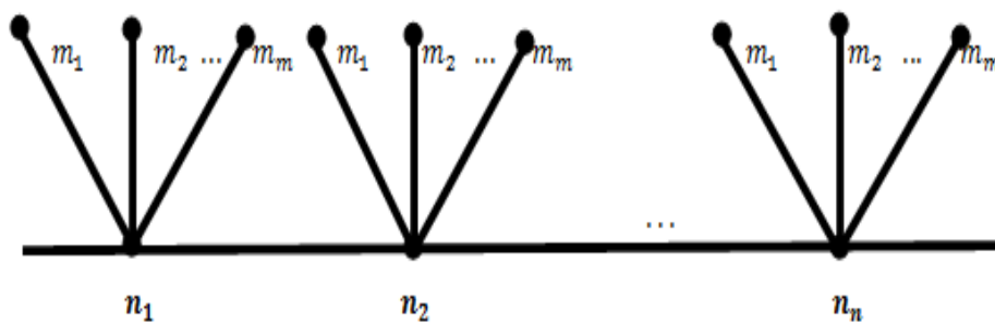
Gambar 2. Graf C_{n,m}
